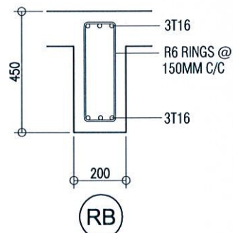
ROOF BEAM DETAILS SCALE 1:20
