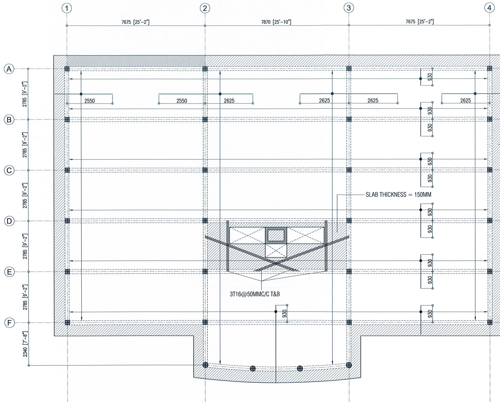
1ST FLOOR SLAB RFMT PLAN SCALE - 1:100
