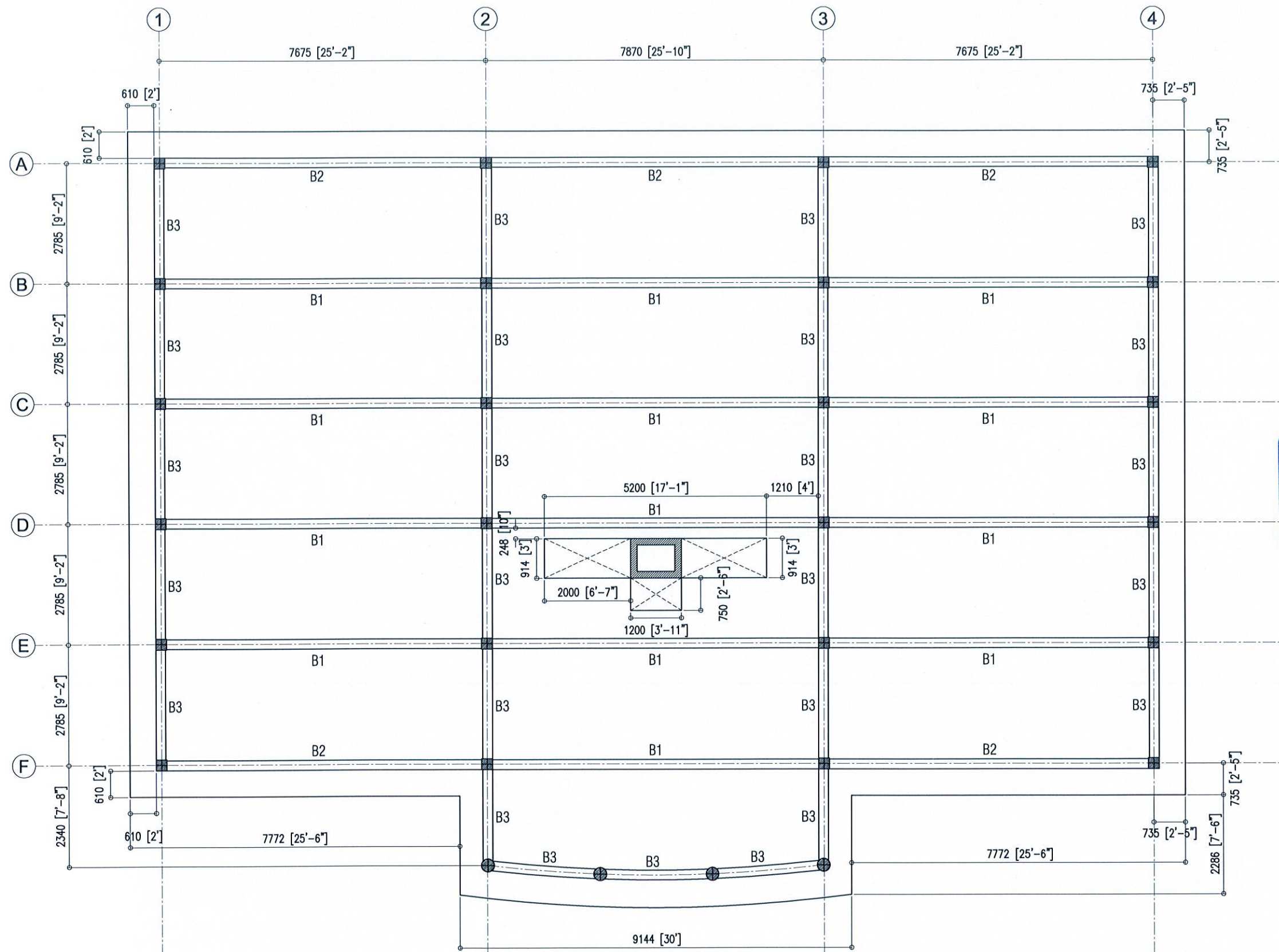
1ST FLOOR BEAM PLAN SCALE - 1:100
