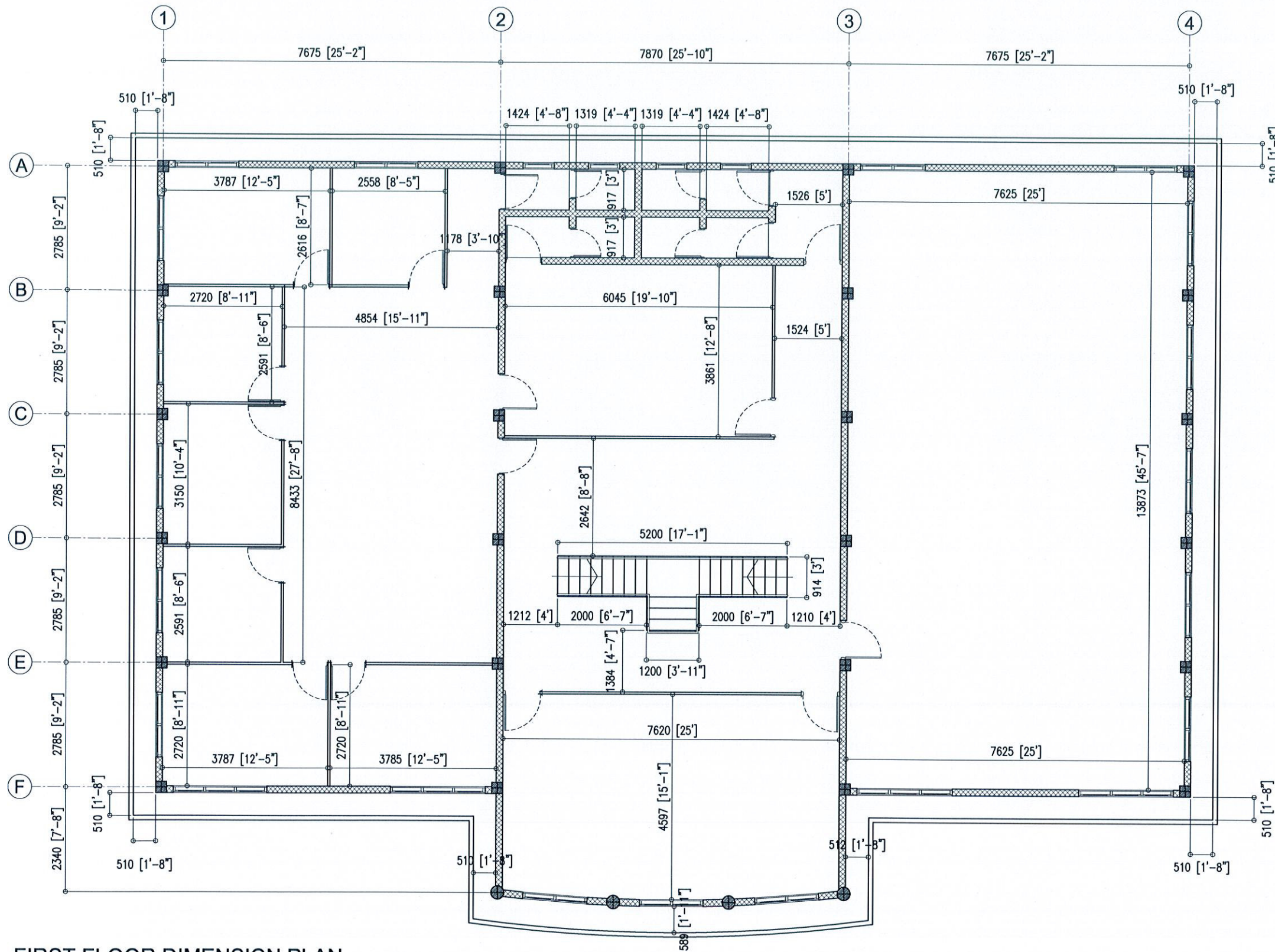
FIRST FLOOR DIMENSION PLAN SCALE - 1:100
