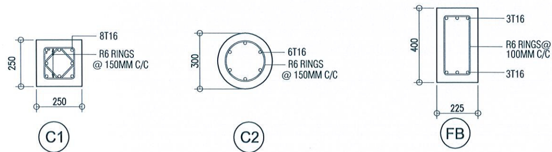
FOUNDATION BEAM AND COLUMN DETAILS SCALE-1:20
