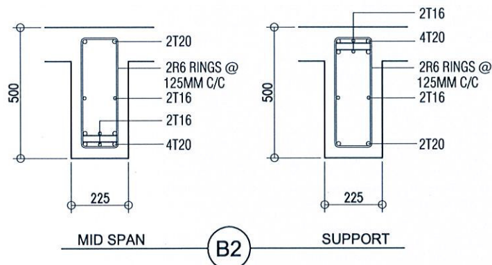
BEAM DETAILS SCALE 1:20
