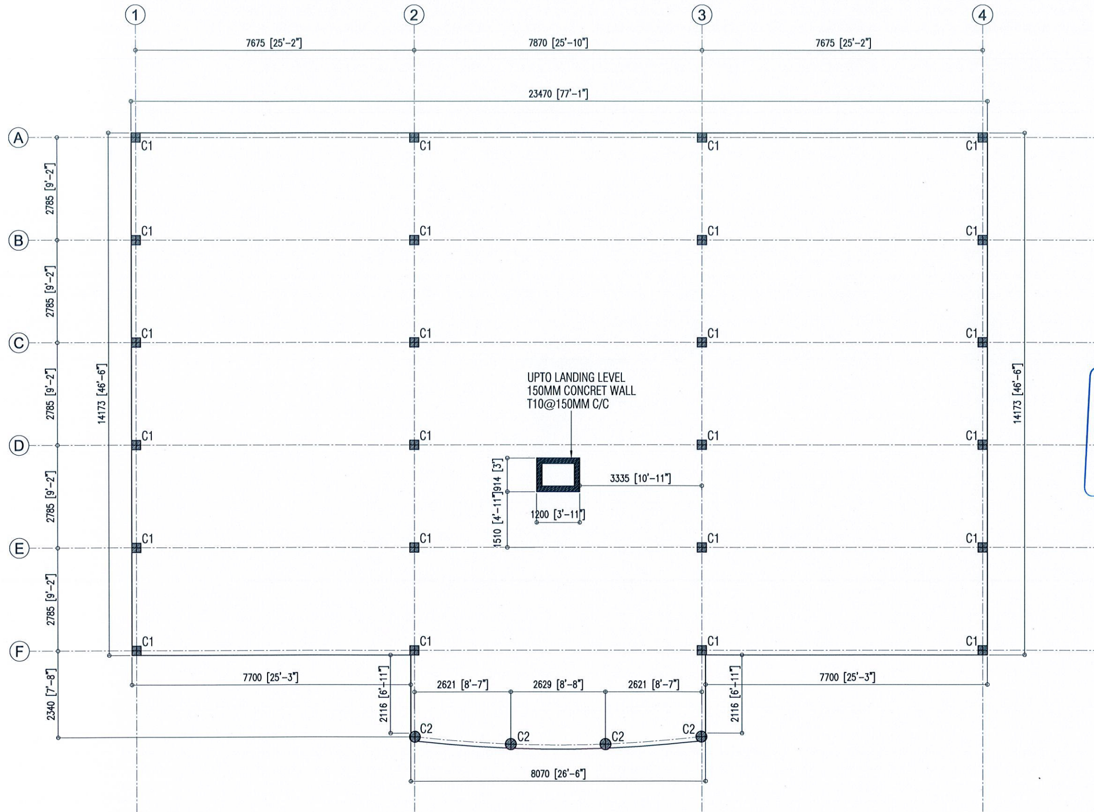
COLUMN SETTING OUT PLAN SCALE - 1:100
