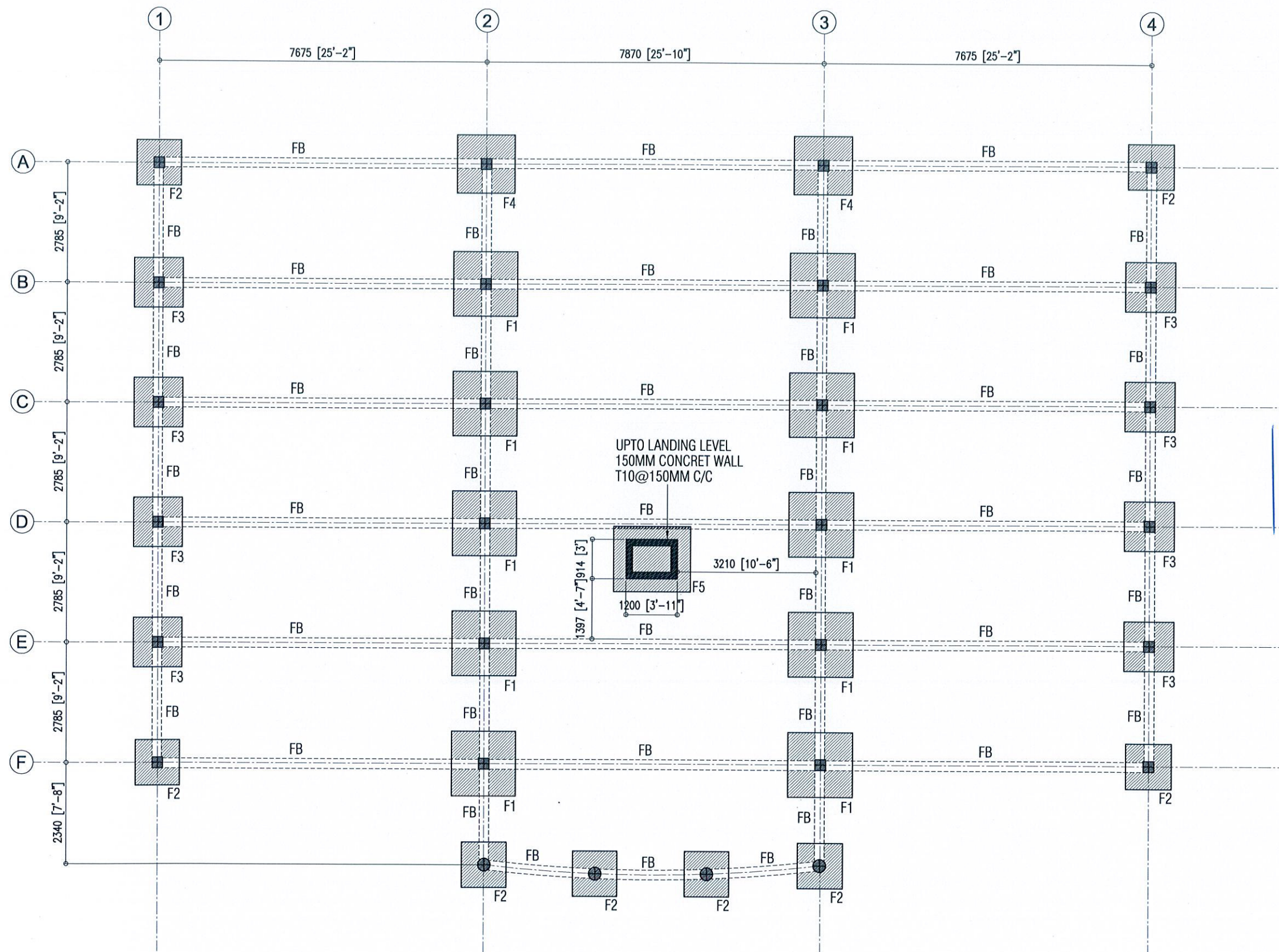
FOUNDATION PLAN SCALE - 1:100
