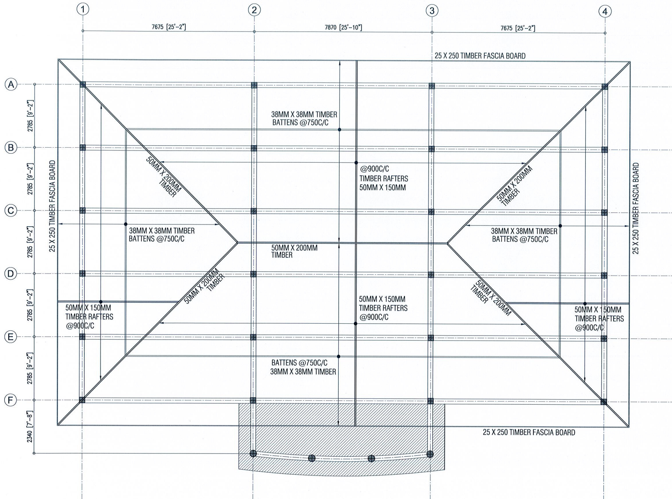
ROOF FRAMING PLAN SCALE - 1:100
