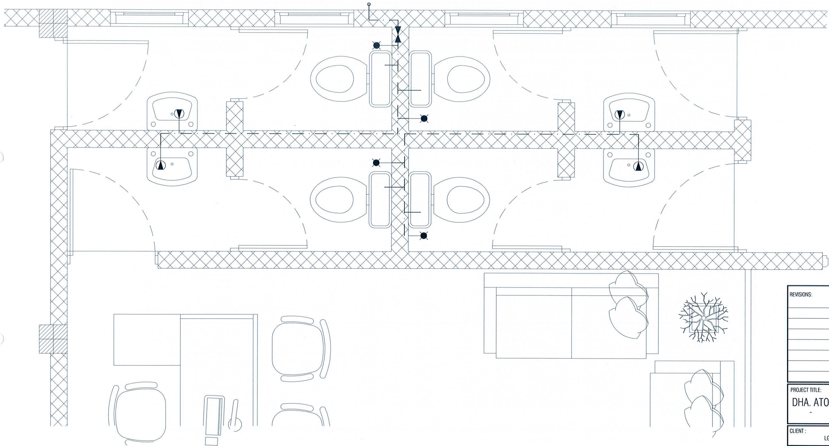
GROUND WATER SUPPLY LAYOUT - TYPE-1 SCALE - 1:20
