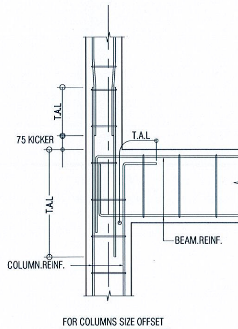
TYPICAL JUNCTION DETAILS OF BEAM & COLUMN SCALE 1:20
