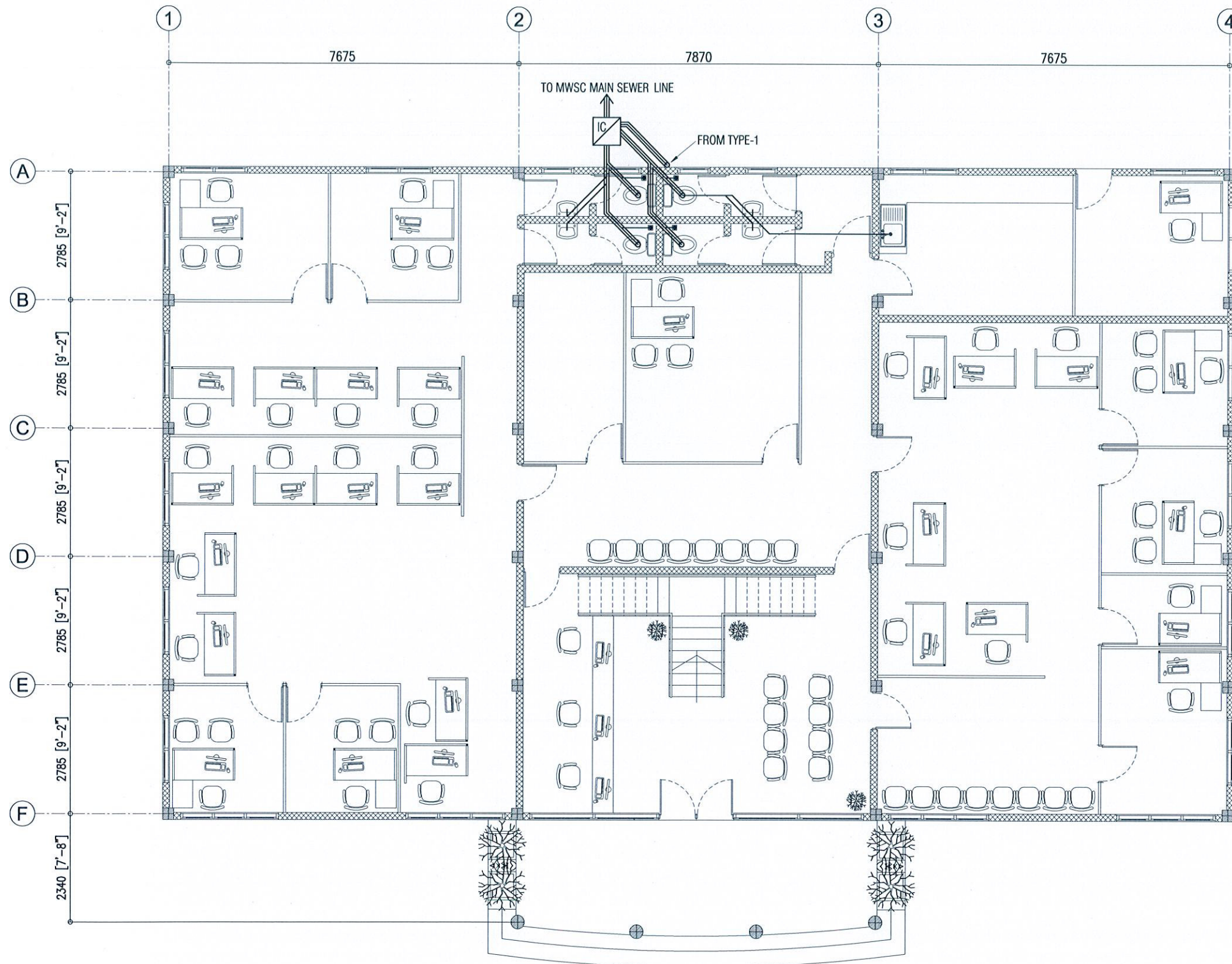
GROUND FLOOR WASTE WATER LINE LAYOUT SCALE - 1:100
