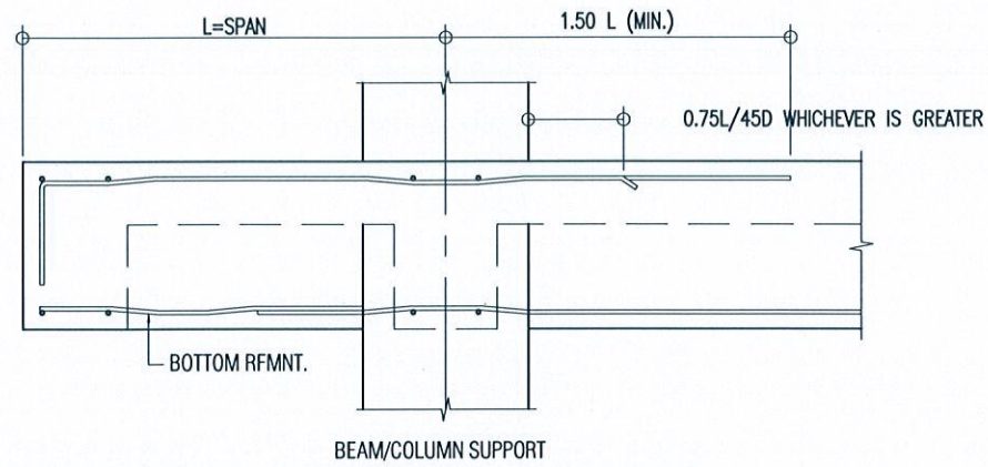
TYPICAL BEAM DETAILS FOR CANTILEVER SCALE 1:20
