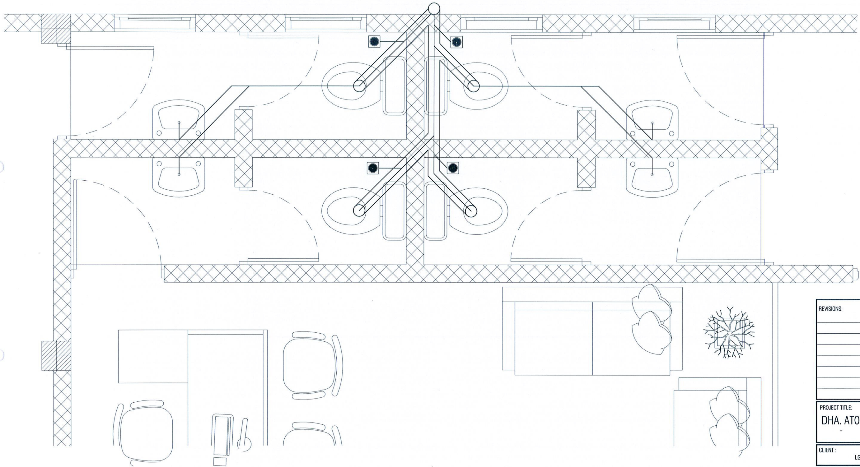
WASTE WATER AND SEWAGE DISPOSAL LAYOUT - TYPE-1 SCALE - 1:20
