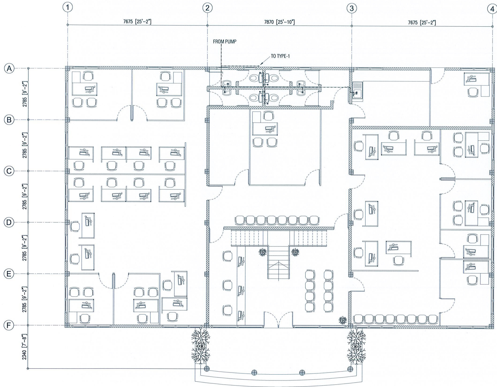
GROUND FLOOR WELL WATER LINE LAYOUT SCALE - 1:100
