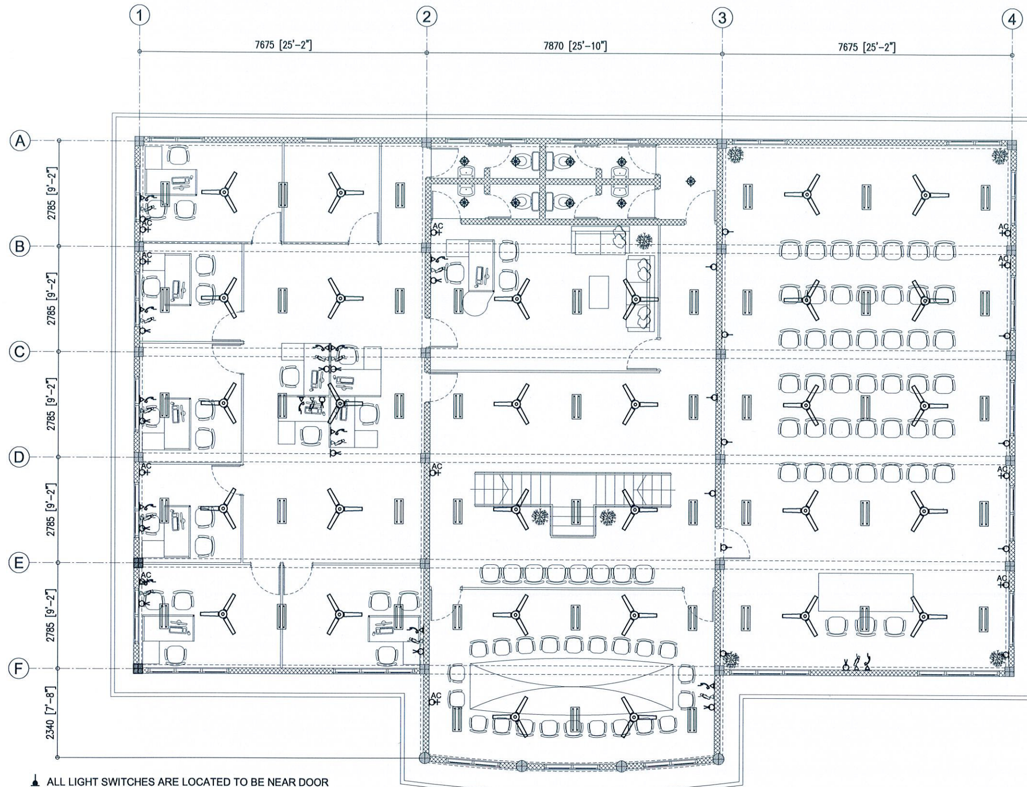
1ST FLOOR ELECTRICAL LAYOUT SCALE - 1:100
