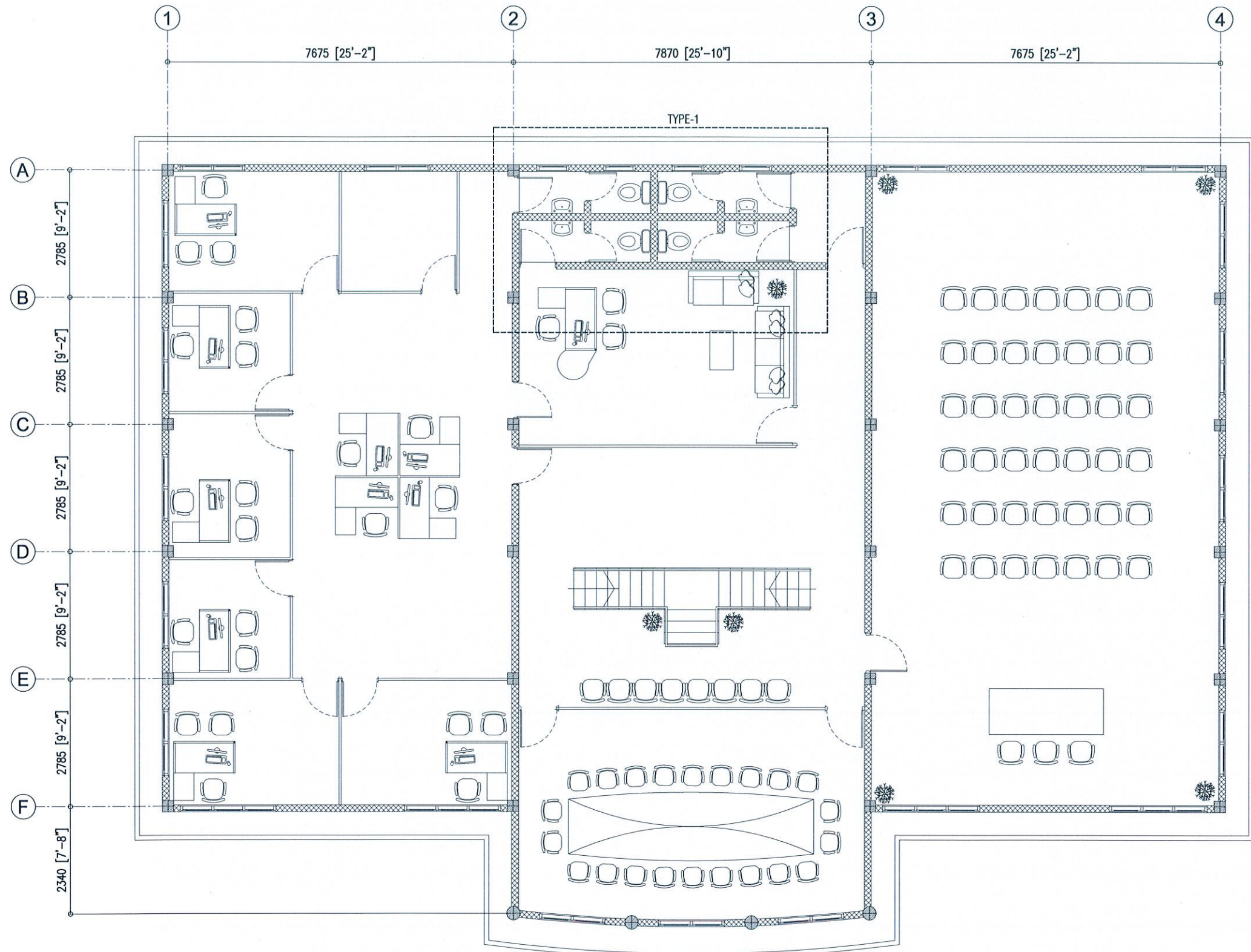
1ST FLOOR KEY PLAN SCALE - 1:100
